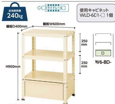
W6-BD-IV W6-BD- 質量:23.2kg ¥66,240
