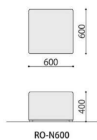
RO-N600
