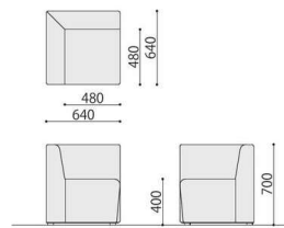
RO-SC90
