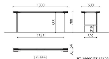
BT-1860S/BT-1860B
