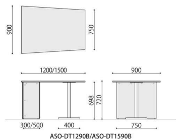
ASO-DT1290B(WH)
