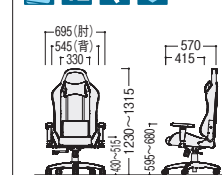
AGC-320F
